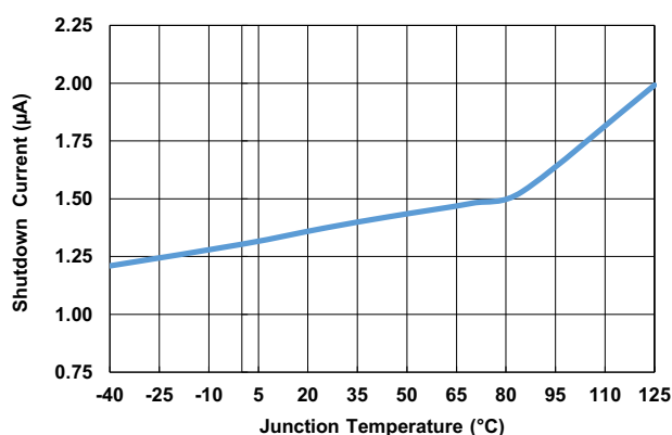
Figure 5. PVIN Shutdown Current vs Junction Temperature
