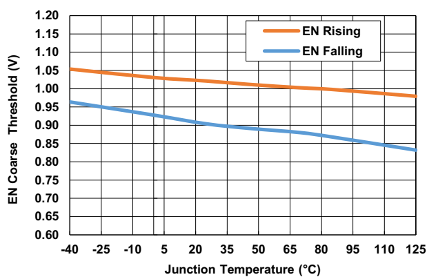
Figure 7. Enable Coarse Threshold vs Junction Temperature
