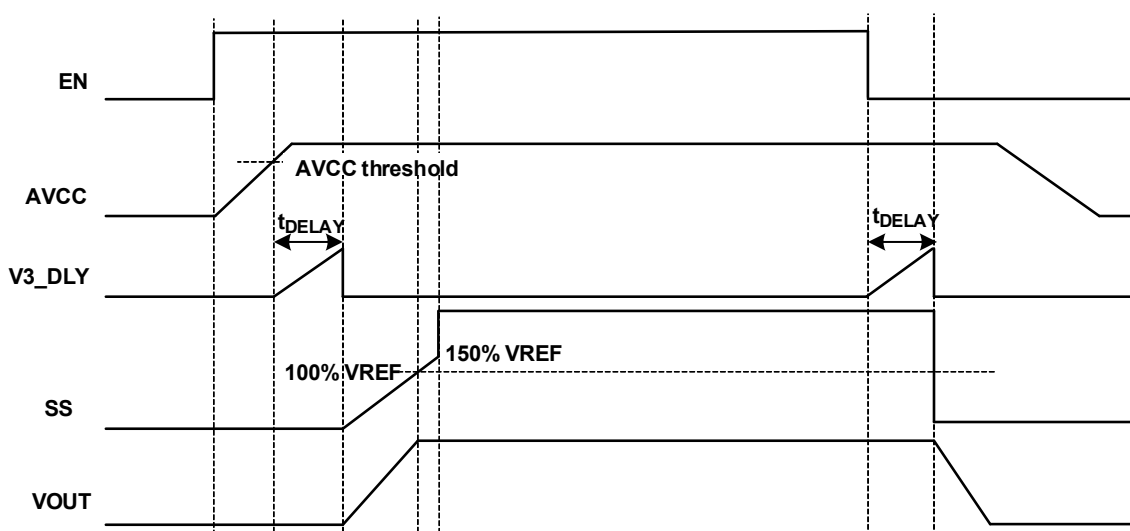
Figure 55. Delay Function
