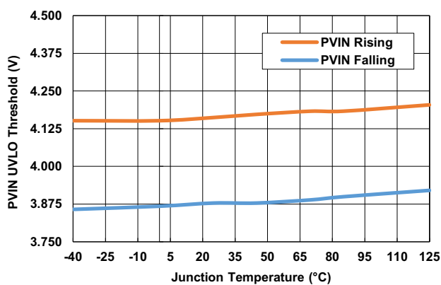
Figure 9. PVIN UVLO Threshold vs Junction Temperature
