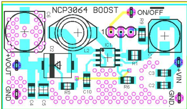
Figure 21. Boost Demoboard Layout
