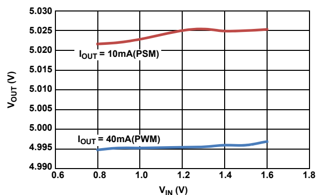
FIGURE 14. LINE REGULATION, V_{OUT} = 5.0
