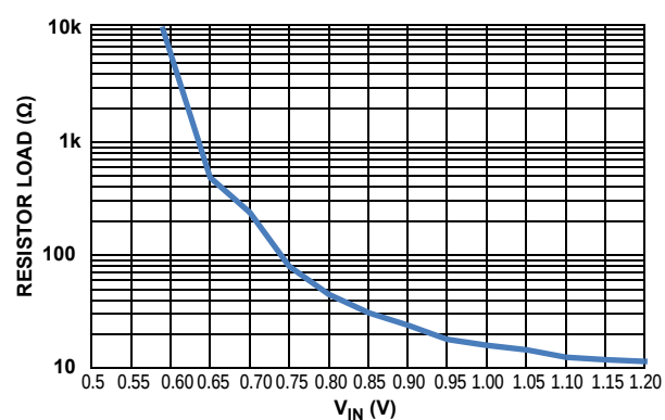
FIGURE 16. START-UP WITH MINIMUM RESISTANCE (PRELOADED) vs V_{IN}
