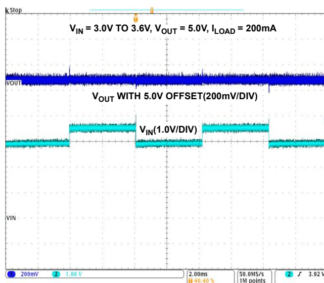
FIGURE 23. LINE TRANSIENT
