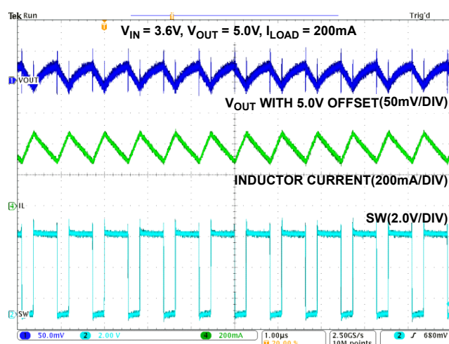
FIGURE 18. PWM WAVEFORM
