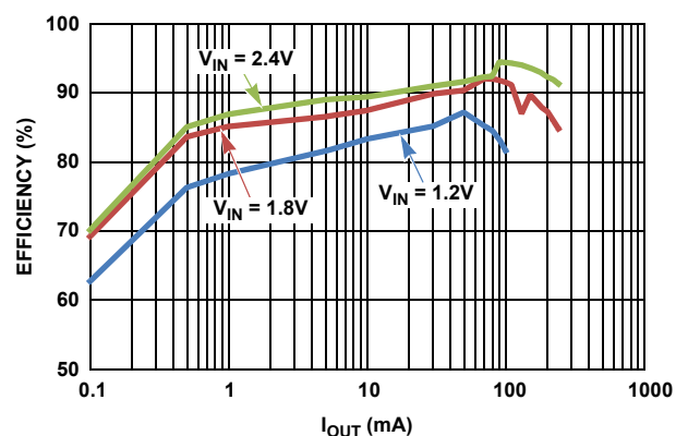
FIGURE 8. EFFICIENCY AT V_{OUT} = 3.3V
