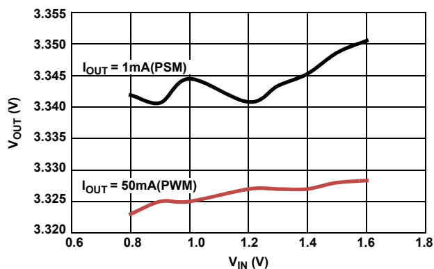
FIGURE 12. LINE REGULATION, V_{OUT} = 3.3V
