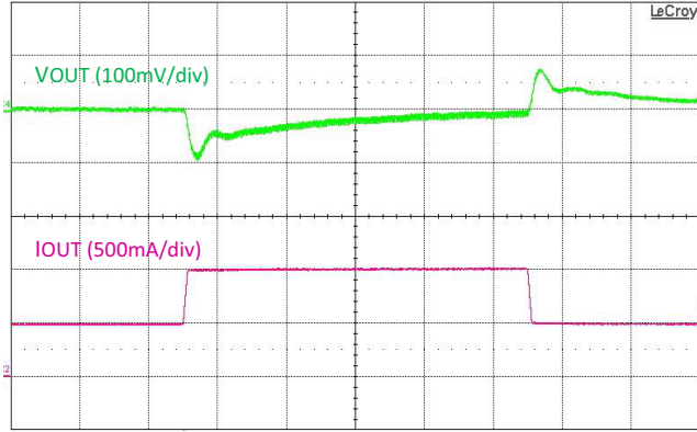
Figure 17. Load Transient, I_{OUT} = 500 \leftrightarrow 1000\text{ mA} , 1\text{ }\mu\text{s} Edge
