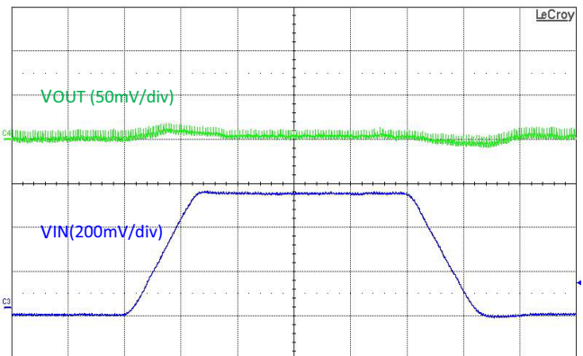
Figure 20. Line Transient, V_{IN} = 2.5\text{ V} \leftrightarrow 3.0\text{ V} , 10\text{ }\mu\text{s} Edge, I_{OUT} = 300\text{ mA}
