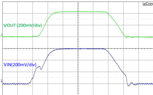
Figure 19. Line Transient, V_{IN} = 3.0\text{ V} \leftrightarrow 3.6\text{ V} , 10\text{ }\mu\text{s} Edge, I_{OUT} = 500\text{ mA} , V_{OUT} = 3.15\text{ V}
