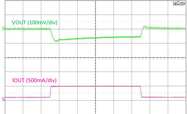
Figure 18. Load Transient, I_{OUT} = 100 \leftrightarrow 500\text{ mA} , 1\text{ }\mu\text{s} Edge, V_{OUT} = 3.15\text{ V}
