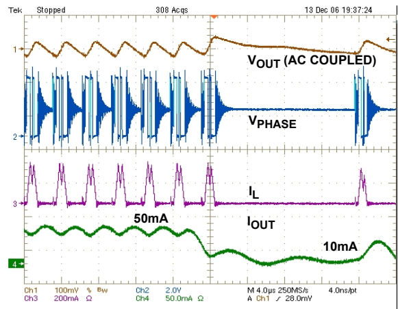
FIGURE 13. (PFM, V_{\text{IN}} = 3.6\text{V} , V_{\text{OUT}} = 1.6\text{V} )
