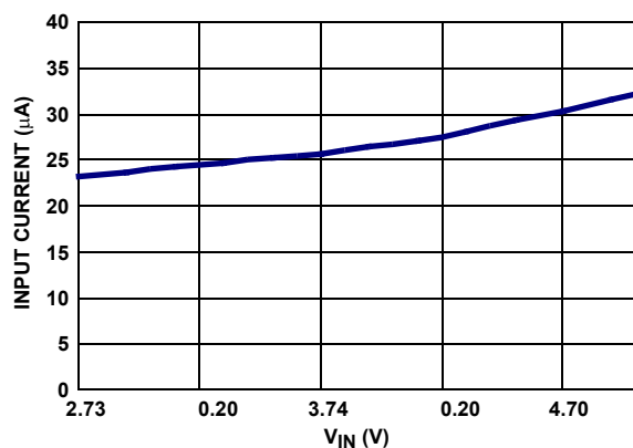
FIGURE 5. I_{\text{Q}} vs V_{\text{IN}} (PFM)
