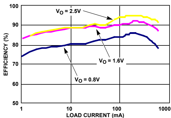
FIGURE 1. EFFICIENCY vs LOAD CURRENT ( V_{\text{IN}} = 3.6\text{V} )
