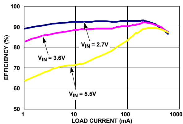
FIGURE 2. EFFICIENCY vs LOAD CURRENT ( V_{\text{O}} = 1.6\text{V} )
