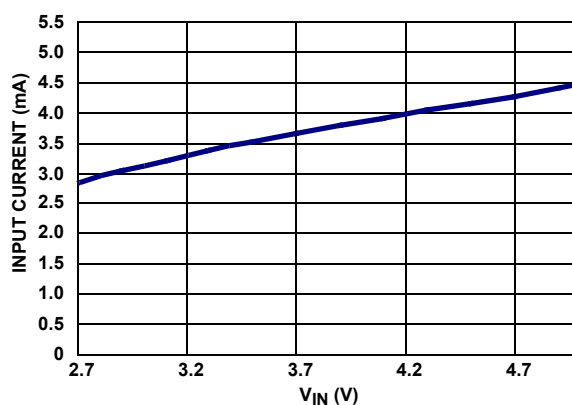
FIGURE 6. I_{\text{Q}} vs V_{\text{IN}} (PWM)
