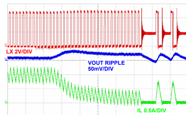
FIGURE 18. MODE TRANSITION CCM TO DCM, (5μs/DIV)
