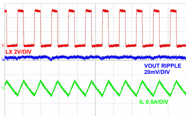
FIGURE 15. STEADY STATE OPERATION AT NO LOAD (PWM), (1μs/DIV)
