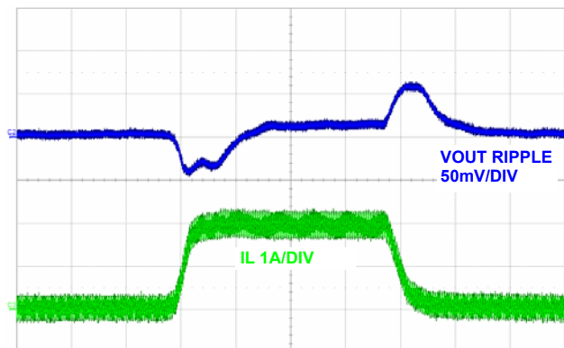
FIGURE 20. LOAD TRANSIENT (PWM), (50μs/DIV)
