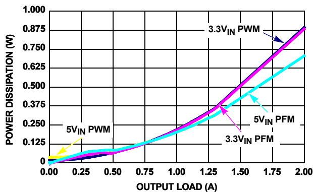
FIGURE 7. POWER DISSIPATION vs LOAD (1MHz, V_{\text{OUT}} = 1.8\text{V} )
