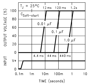
Soft-start Response
