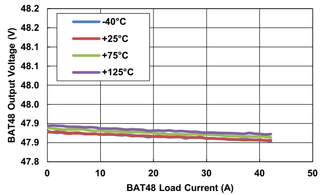
Figure 97. BAT48 Voltage in Boost/FPWM/NO-PD with Temperature Variable, f_{CLK} = 100\text{kHz}
