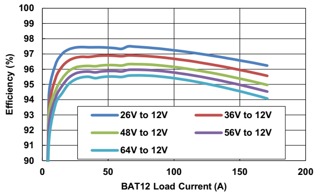
Figure 8. Buck Efficiency (4-Phase, Buck Mode, DE Mode, Phase Drop Enabled, f_{CLK} = 100\text{kHz} )
