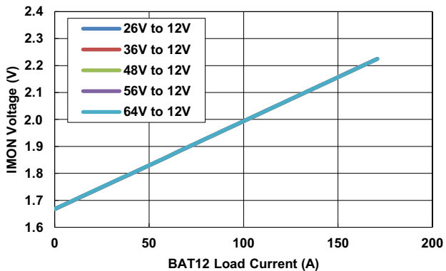
Figure 12. Buck IMON Voltage (+25°C, 4-Phase, Buck Mode, DE Mode, Phase Drop Enabled, f_{CLK} = 100\text{kHz} )
