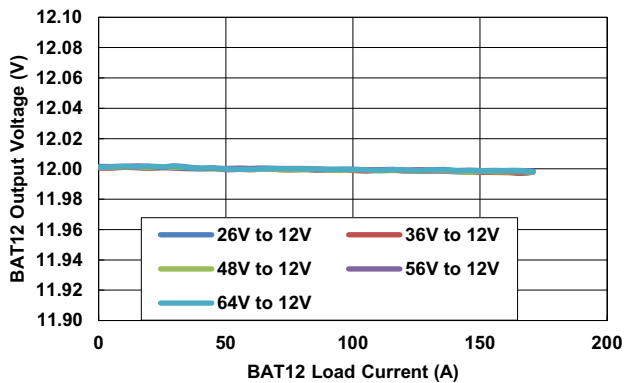
Figure 10. BAT12 Output Voltage (+25°C, 4-Phase, Buck Mode, DE Mode, Phase Drop Enabled, f_{CLK} = 100\text{kHz} )
