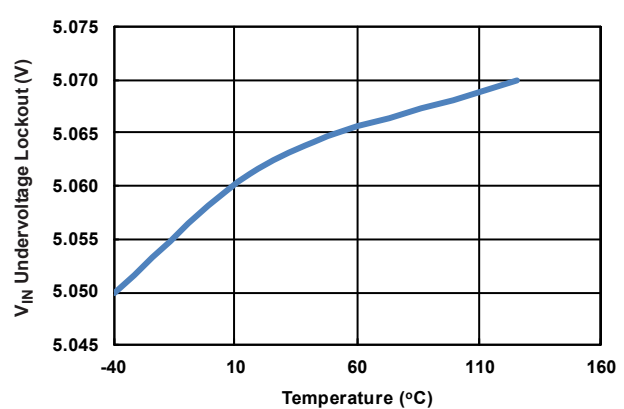
Figure 107. V_{IN} Undervoltage Lockout vs Temperature, Default Register Setting
