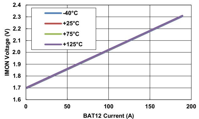
Figure 13. Boost IMON Voltage, BAT12 = 12V (4-Phase, Boost Mode, DE Mode, Phase Drop Enabled, f_{CLK} = 100\text{kHz} )
