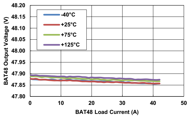
Figure 96. BAT48 Voltage in Boost/FPWM/PD with Temperature Variable, f_{CLK} = 100\text{kHz}
