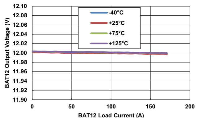
Figure 11. BAT12 Output Voltage (48V IN , 4-Phase, Buck Mode, DE Mode, Phase Drop Enabled, f_{CLK} = 100\text{kHz} )
