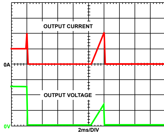
FIGURE 19. OVERCURRENT BEHAVIOR IN HICCUP MODE F_{SW} = 500kHz
