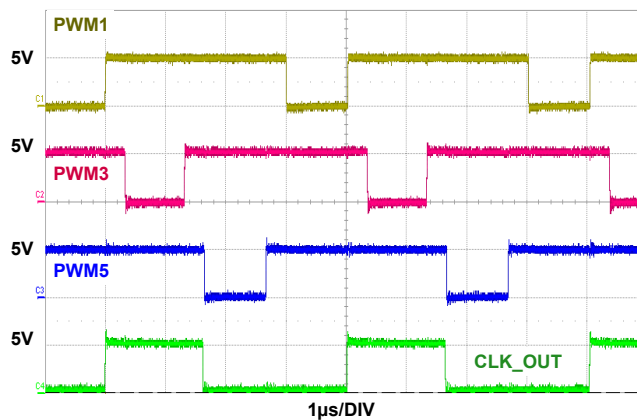
FIGURE 9. WAVEFORMS WITH PWM_INV = VCC
