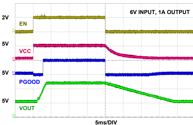
FIGURE 11. ENABLE/DISABLE WAVEFORMS
