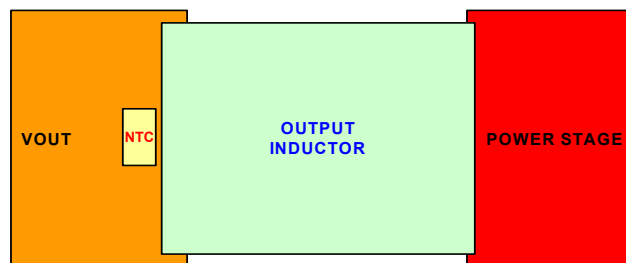
FIGURE 19. RECOMMENDED PLACEMENT OF NTC
