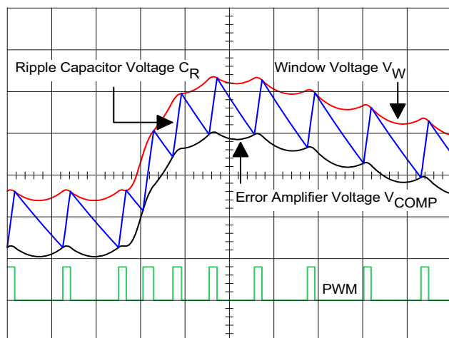
FIGURE 1. MODULATOR WAVEFORMS DURING LOAD TRANSIENT
