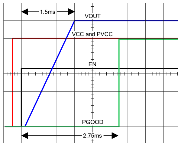
FIGURE 2. SOFT-START SEQUENCE
