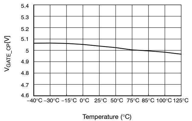
Figure 8. V GATE_CP vs. Temperature
