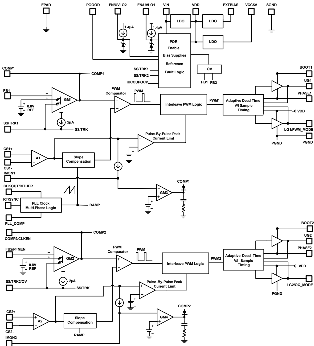
Figure 5. Block Diagram
