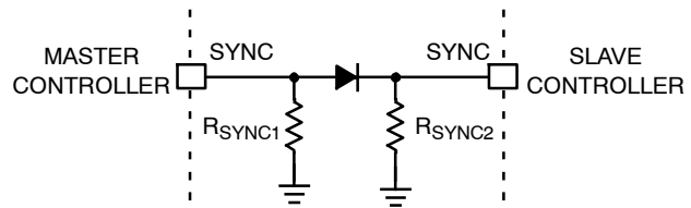
Figure 50. Master-Slave Configuration
