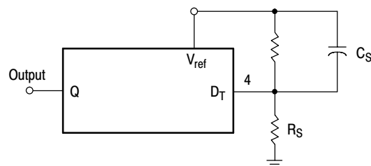
Figure 17. Soft-Start Circuit
