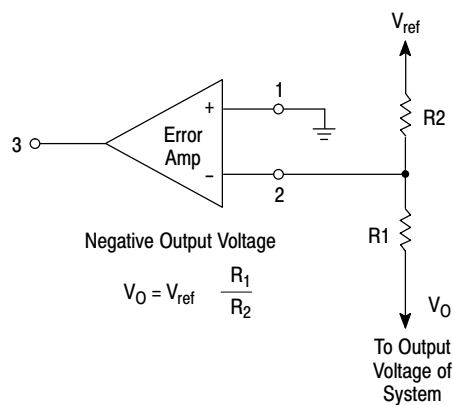
Figure 15. Error-Amplifier Sensing Techniques
