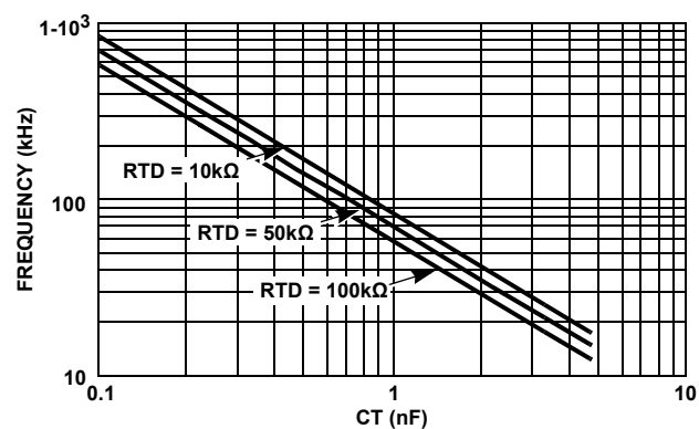
FIGURE 9. CAPACITANCE vs FREQUENCY
