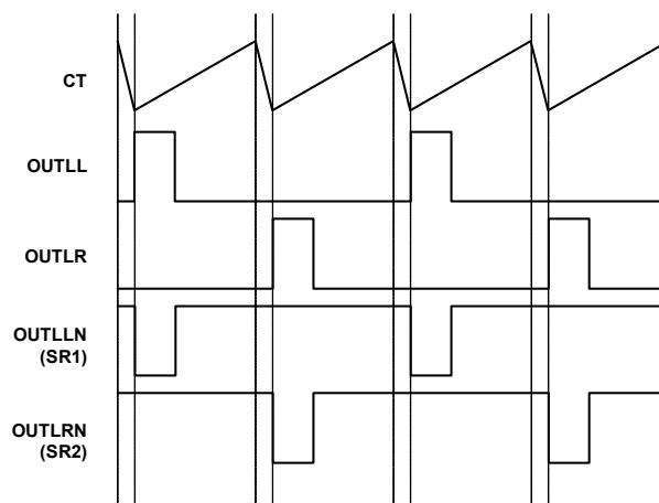
FIGURE 25. BASIC WAVEFORM TIMING
