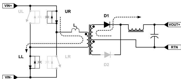
FIGURE 22. UR - L_p POWER TRANSFER CYCLE
