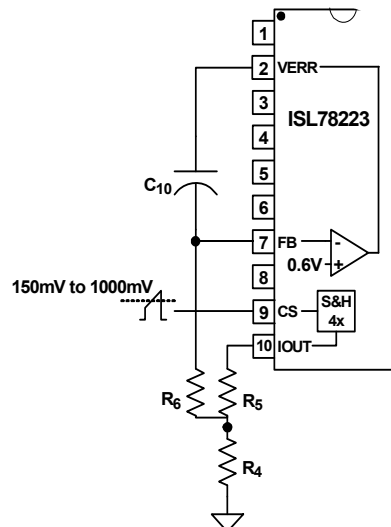
FIGURE 12. AVERAGE OVERCURRENT IMPLEMENTATION
