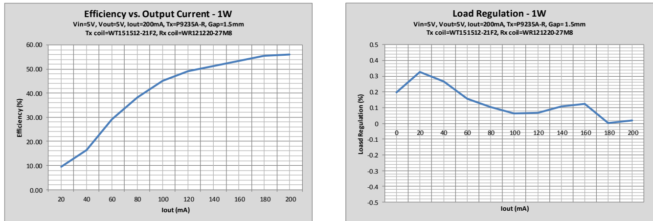
Figure 4. Typical Performance Characteristics – 1W
