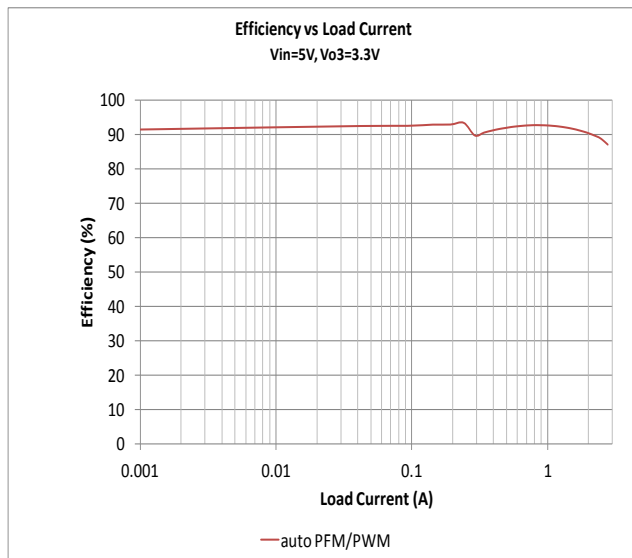
Figure 9. Channel 3 Efficiency
