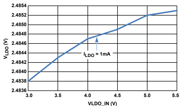
FIGURE 11. LDO LINE REGULATION vs V_{IN}
