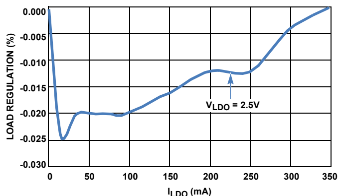
FIGURE 12. LDO LOAD REGULATION vs I_{LDO}
