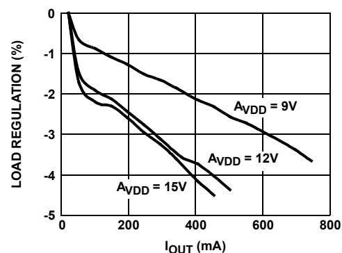
FIGURE 8. V_{\text{BOOST}} LOAD REGULATION AT V_{\text{IN}} = 5\text{V} (P-MODE)
