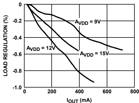
FIGURE 6. V_{\text{BOOST}} LOAD REGULATION AT V_{\text{IN}} = 5\text{V} (PI-MODE)
