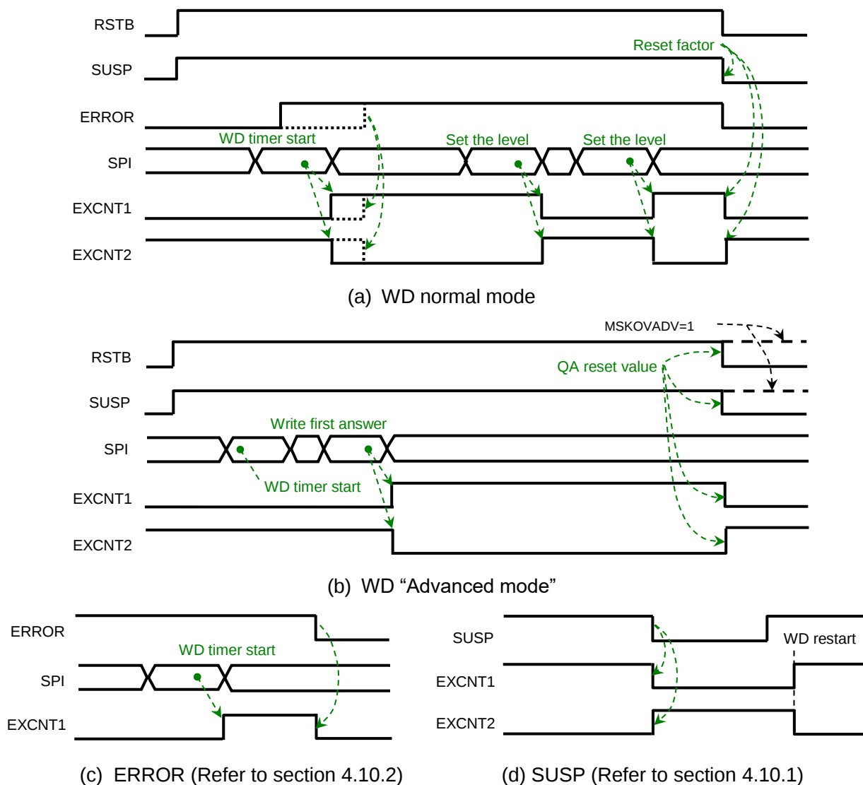
Figure 4-44 EXCNT1/2 operation
