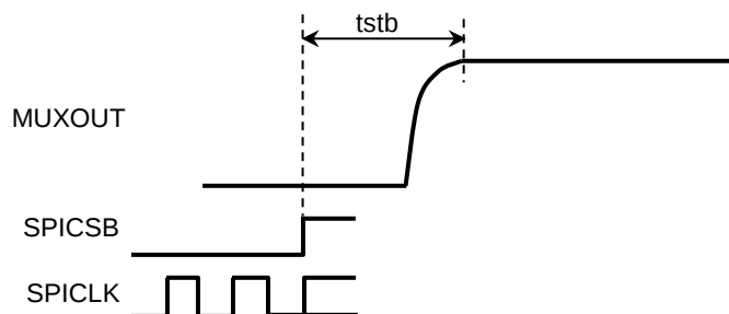
Figure 4-56 Output timing
