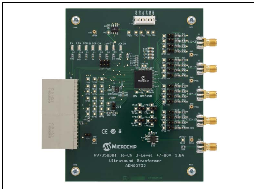
FIGURE 1-1: HV7358DB1 Board Photo.
