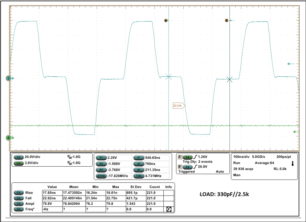
FIGURE C-5: Rise Fall Time of \pm 80V , 5 MHz RTZ, 330 pF//2.5K Load.
