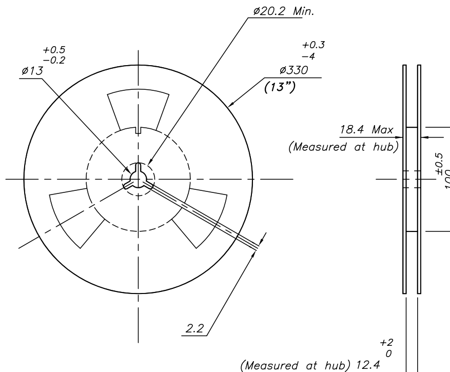
Figure 67. Reel outline
