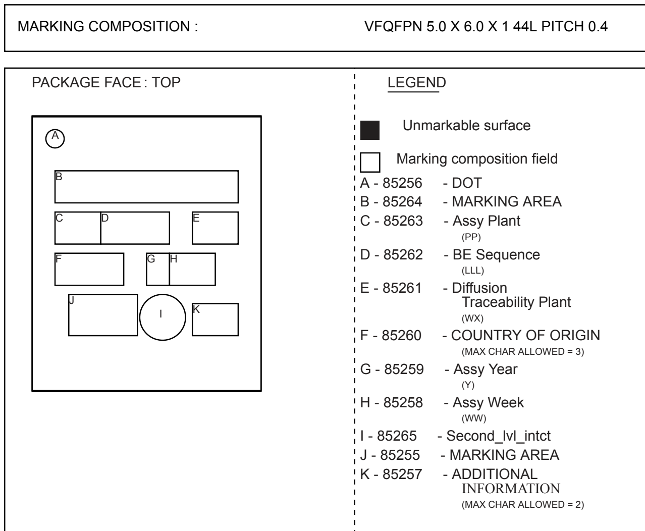
Figure 68. Marking composition
