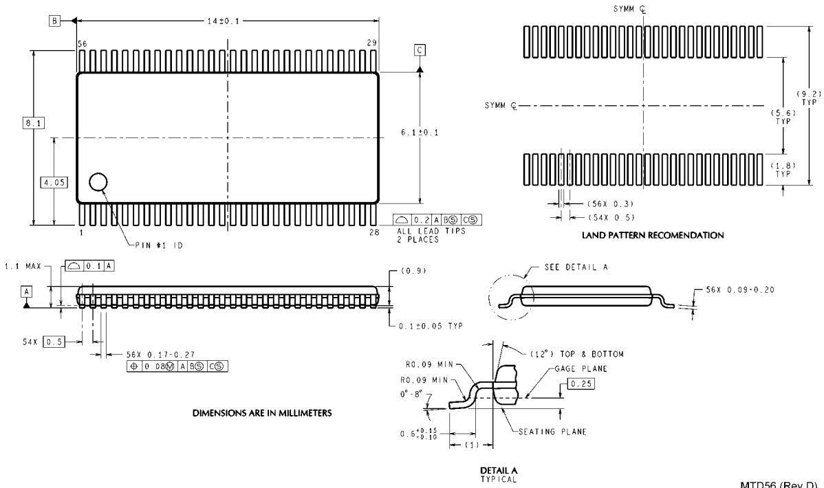
56-Lead Molded TSSOP Package, JEDEC Registration Number MO-153 Variation EE, Order Number LM94C1MT or LM94C1MTX, NS Package Number MTD56
