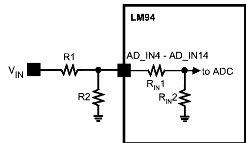
FIGURE 3. AD_IN4 - AD_IN14 External Resistor Divider
