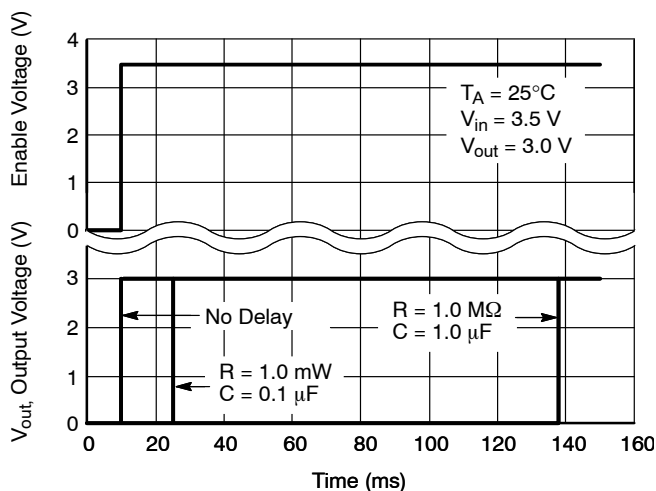
Figure 21. Delayed Turn-on
