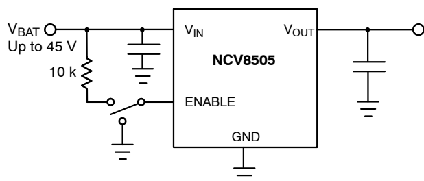
Figure 16. ENABLE Function
