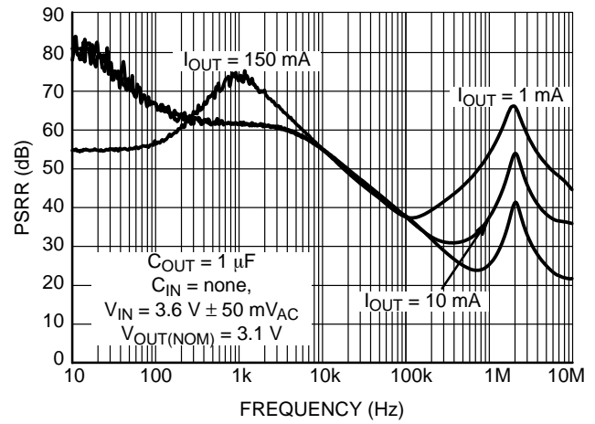
Figure 46. PSRR vs. Frequency V_{OUT} = 3.1 \text{ V}
