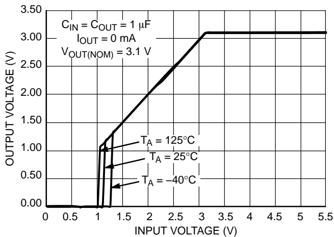
Figure 19. Output Voltage vs. Input Voltage V_{OUT} = 3.1\ \text{V}
