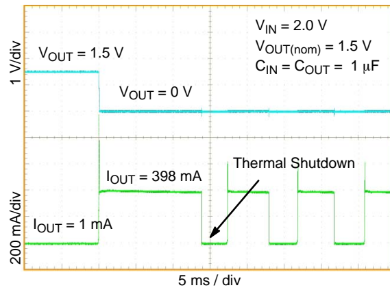
Figure 67. Short-Circuit Response V_{OUT} = 1.5 V, C_{OUT} = 1 \mu F
