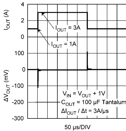
Load Transient Response, C_{OUT} = 100 \mu F Tantalum
