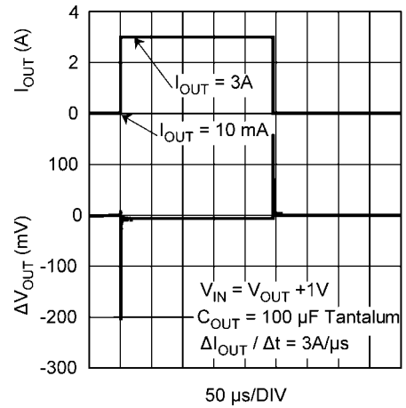
Load Transient Response, C_{OUT} = 100 \mu F Tantalum
