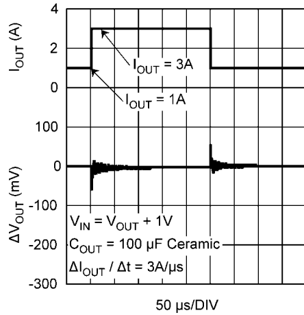
Load Transient Response, C_{OUT} = 100 \mu F Ceramic
