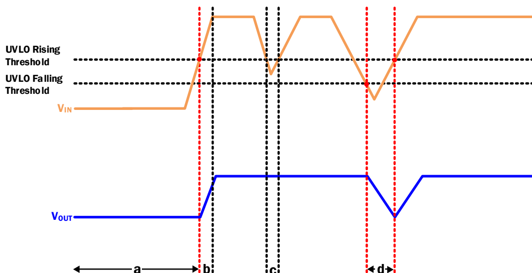
Figure 75. UVLO Operation
