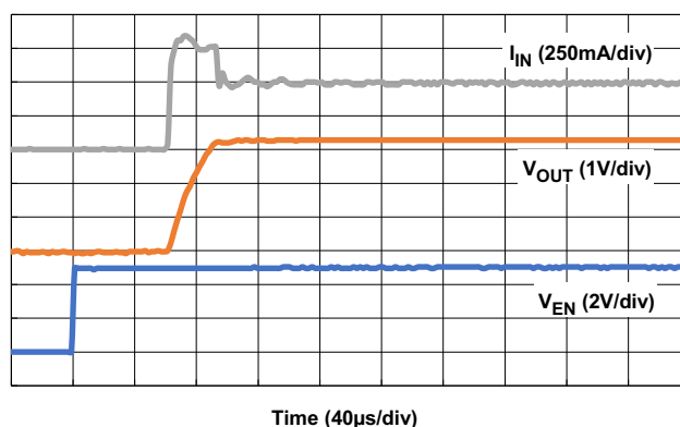
Figure 26. Start-Up and In-Rush Current ( V_{IN} = 4.3V , V_{OUT} = 3.3V , I_{OUT} = 500mA , C_{FF} = 22pF , C_{OUT} = 2.2\mu F )
