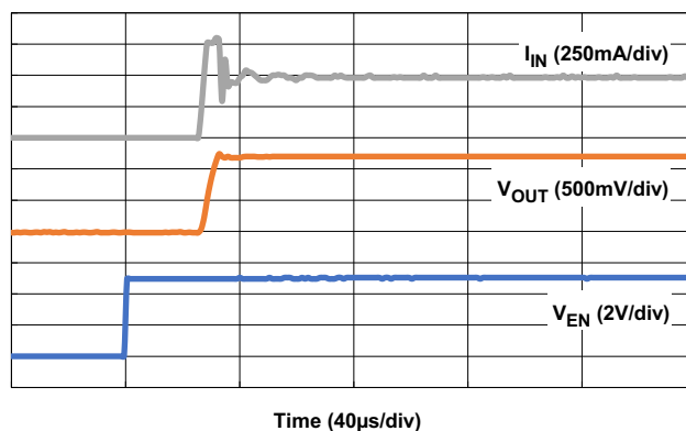
Figure 24. Start-Up and In-Rush Current ( V_{IN} = 2.5V , V_{OUT} = V_{ADJ} , I_{OUT} = 500mA , C_{FF} = \text{None} , C_{OUT} = 2.2\mu F )
