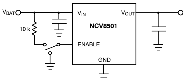
Figure 15. ENABLE Function
