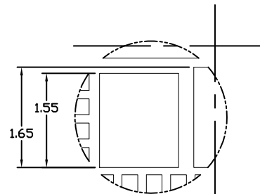
DETAIL F
