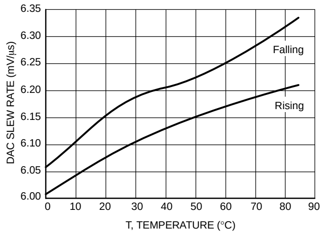
Figure 16. DAC Slew Rate vs. Temperature
