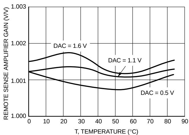
Figure 10. Remote Sense Amplifier Gain vs. Temperature
