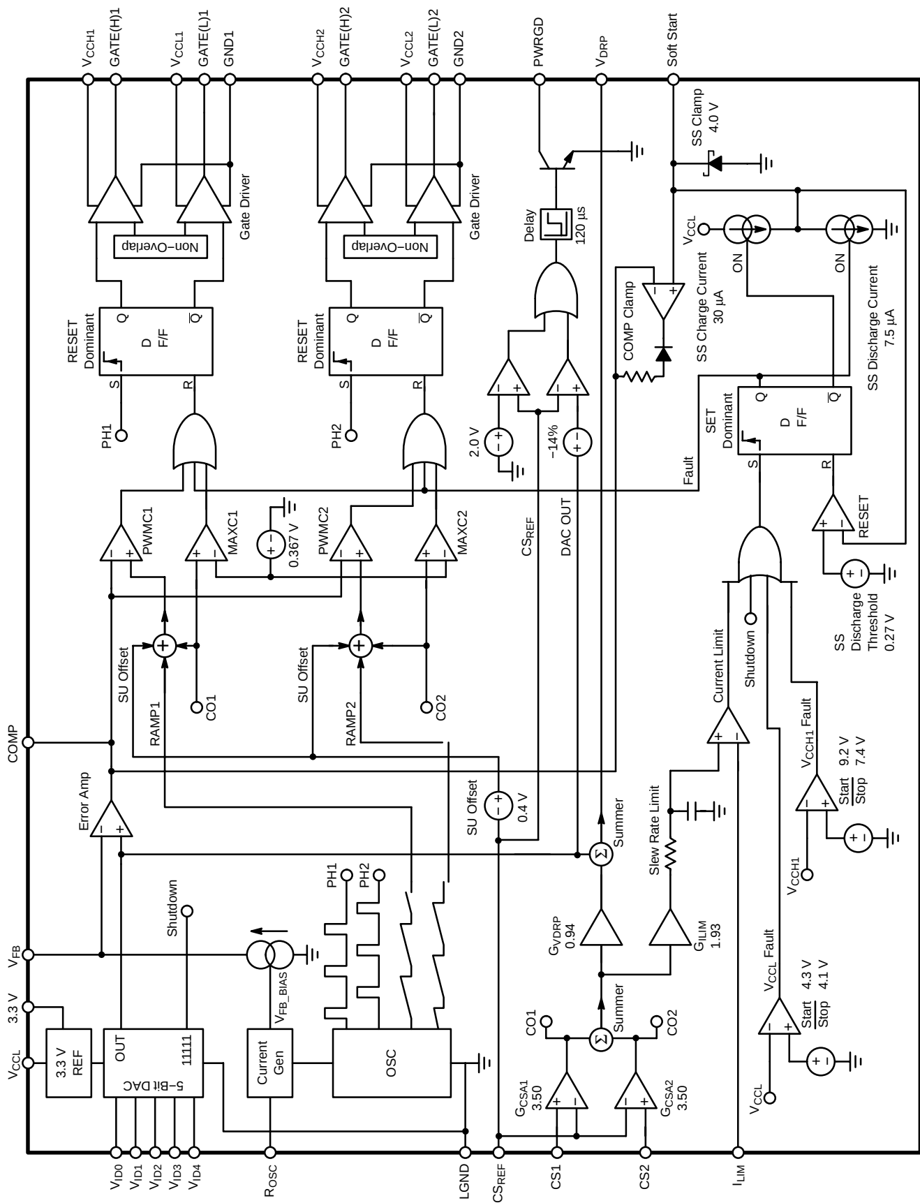
Figure 3. Block Diagram
