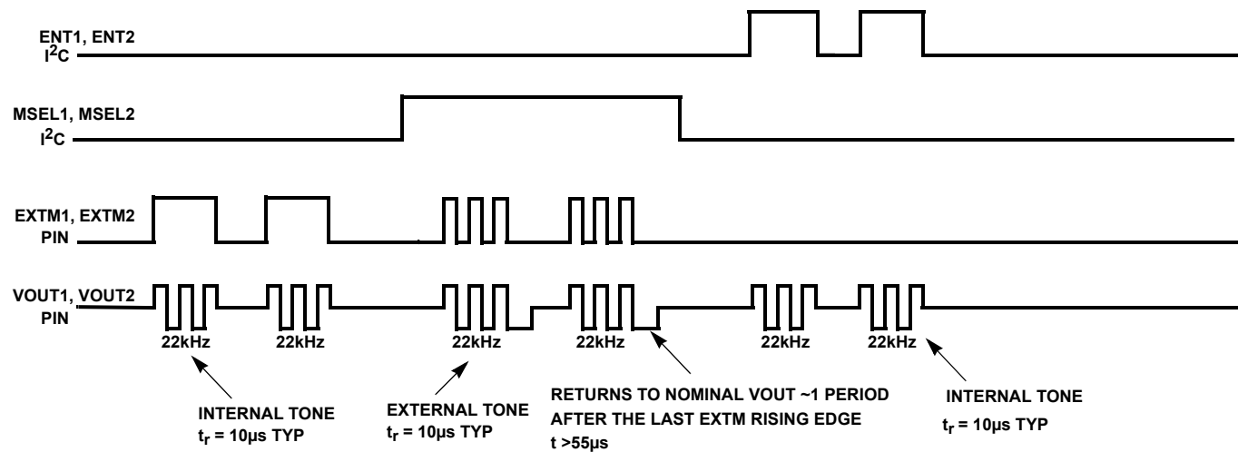
FIGURE 1. TONE WAVEFORM
