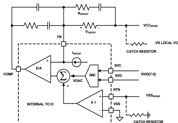
FIGURE 15. DIFFERENTIAL SENSING AND LOAD LINE IMPLEMENTATION
