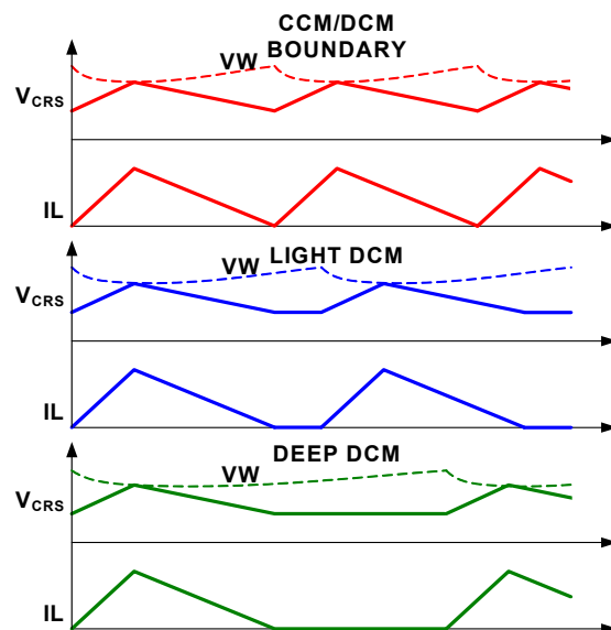
FIGURE 12. PERIOD STRETCHING
