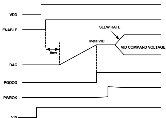
FIGURE 14. TYPICAL SOFT-START WAVEFORMS
