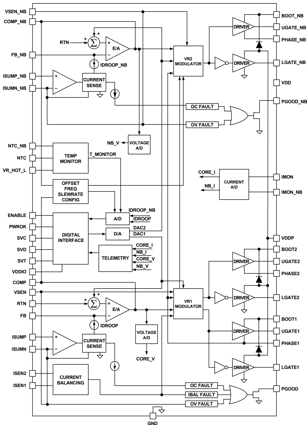
FIGURE 6. BLOCK DIAGRAM
