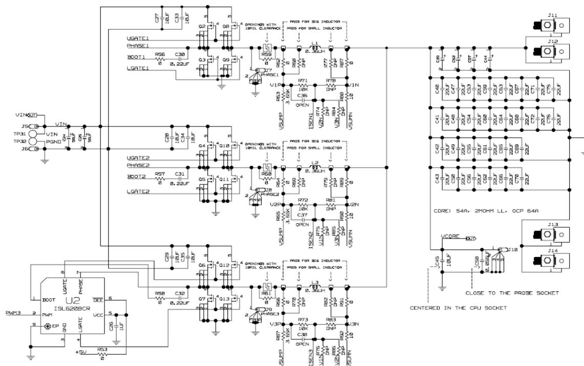
FIGURE 31. PORTION OF ISL6267EVAL1Z EVALUATION BOARD SCHEMATIC
