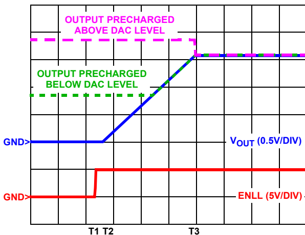
FIGURE 12. SOFT-START WAVEFORMS FOR ISL6308-BASED MULTI-PHASE CONVERTER
