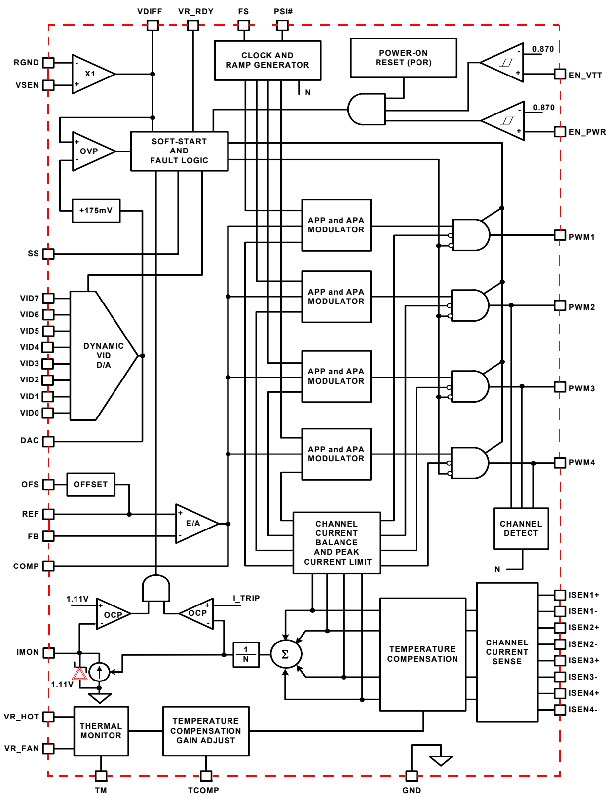
FIGURE 1. BLOCK DIAGRAM
