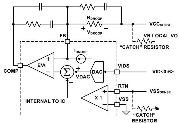
FIGURE 12. DIFFERENTIAL SENSING AND LOAD LINE IMPLEMENTATION
