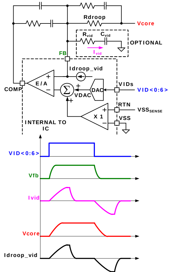
FIGURE 23. OPTIONAL SLEW RATE COMPENSATION CIRCUIT FOR 1-TICK VID TRANSITION
