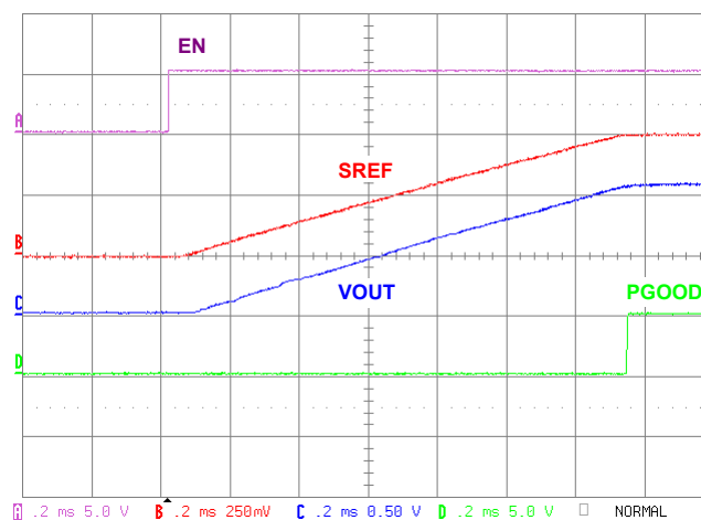
FIGURE 16. START-UP, V_{IN} = 12.6V , V_{OUT} = 1.05V , LOAD = 10A
