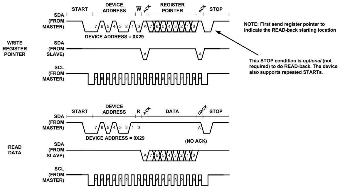
FIGURE 47. I²C READ TIMING DIAGRAM
