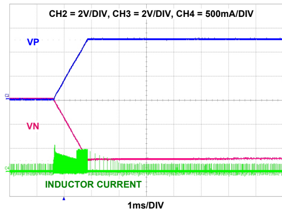
FIGURE 36. VP AND VN ( \pm 5\text{V} ) SOFT-START AT 2.5V INPUT VOLTAGE, VP/VN START TOGETHER (Reg 0x04 <b 4 > = 1)
