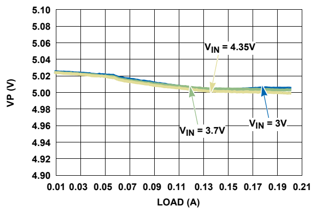
FIGURE 41. VP LOAD REGULATION, 5V
