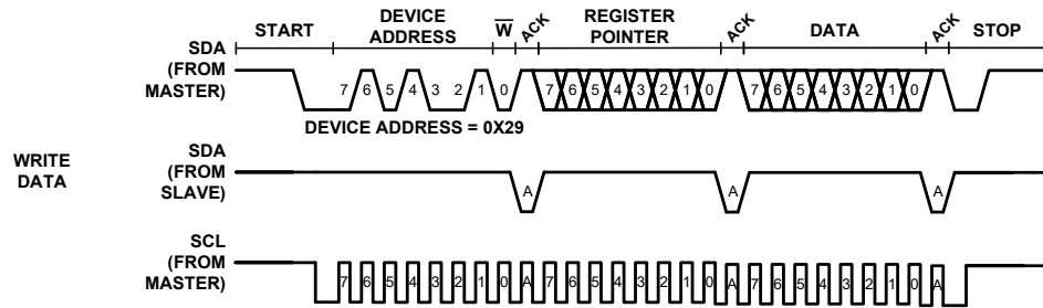
FIGURE 46. I²C WRITE TIMING DIAGRAM
