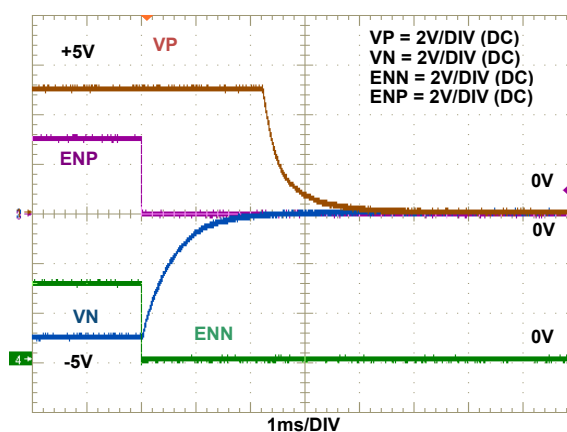
FIGURE 63. OFF SEQUENCE, 1 GPIO CONTROL
