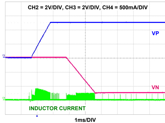
FIGURE 34. VP AND VN ( \pm 5\text{V} ) SOFT-START AT 5V INPUT VOLTAGE, VP/VN SEQUENCED (Reg 0x04 <b 4 > = 0)
