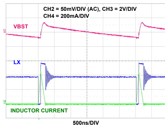
FIGURE 11. VBST RIPPLE, 10mA LOAD, VBST = 5.4V, V_{IN} = 3.7\text{V}
