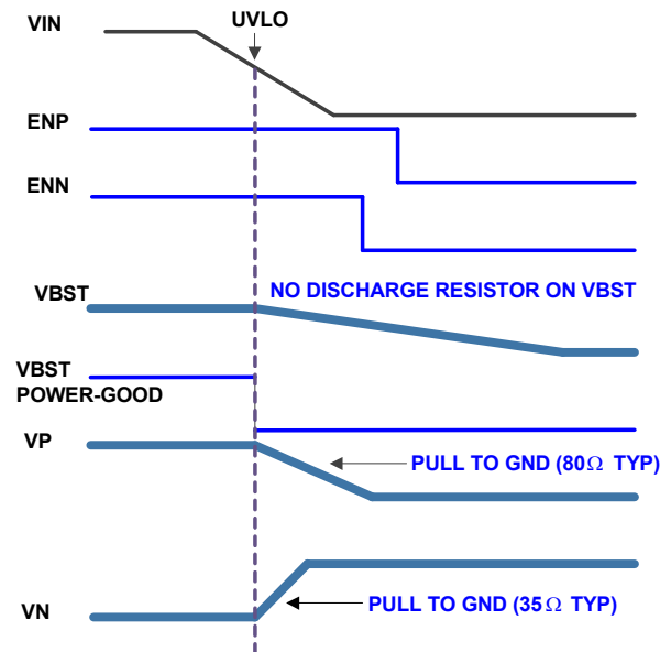
FIGURE 55. POWER-OFF SEQUENCE - ACTIVATED BY VIN FALLING BELOW UVLO
