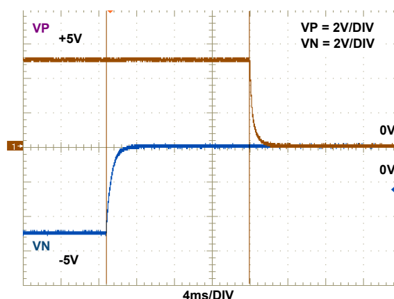
FIGURE 57. OFF SEQUENCE, I 2 C CONTROL
