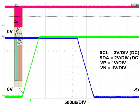
FIGURE 59. I 2 C SEQUENCE AND VP/VN RESPONSE
