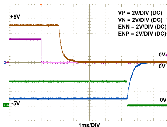
FIGURE 61. OFF SEQUENCE, 2 GPIO CONTROL
