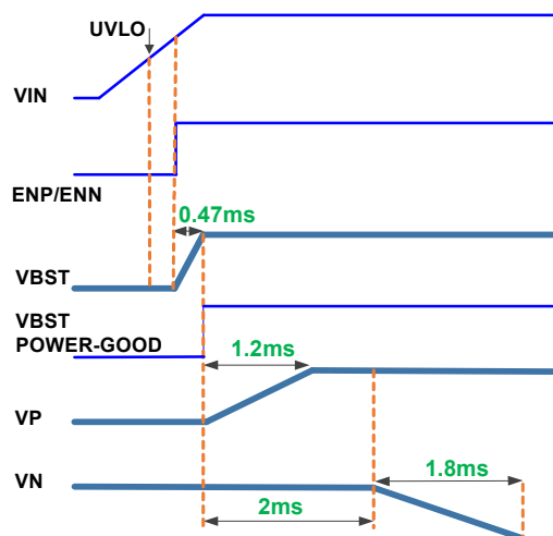
FIGURE 48. POWER-ON SEQUENCE – ACTIVATED BY ONE GPIO FOR ENN AND ENP, REGISTER 0x04 <b 4 > = 0 AND 0x05 <b 7 > = 0
