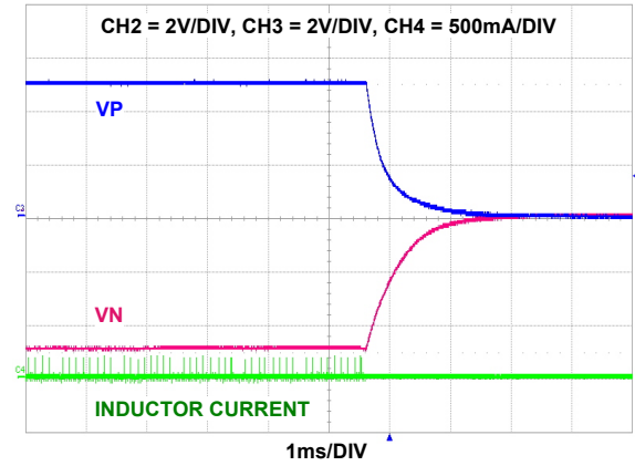
FIGURE 39. VP AND VN ( \pm 5\text{V} ) SHUTDOWN, VP/VN SHUTDOWN TOGETHER (Reg 0x05 <b 4 > = 1)
