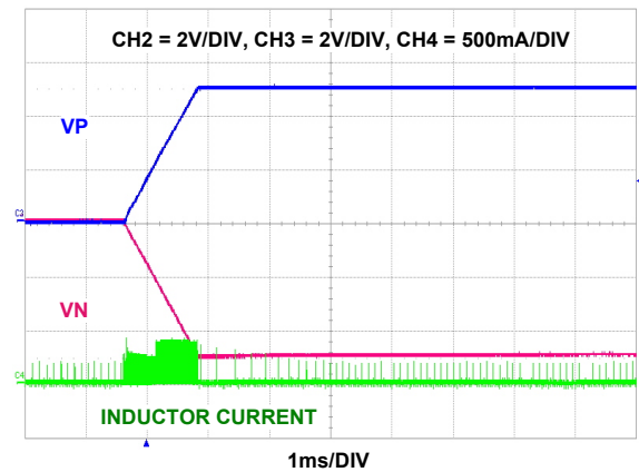
FIGURE 37. VP AND VN ( \pm 5\text{V} ) SOFT-START AT 3.7V INPUT VOLTAGE, VP/VN START TOGETHER (Reg 0x04 <b 4 > = 1)
