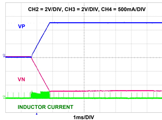
FIGURE 38. VP AND VN ( \pm 5\text{V} ) SOFT-START AT 5V INPUT VOLTAGE, VP/VN START TOGETHER (Reg 0x04 <b 4 > = 1)
