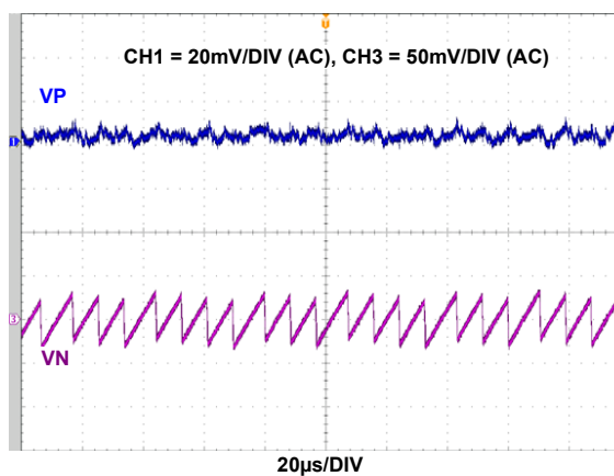
FIGURE 15. VP/VN ( \pm 5\text{V} ) OUTPUT VOLTAGE RIPPLE, 20mA LOAD, V_{IN} = 3\text{V}
