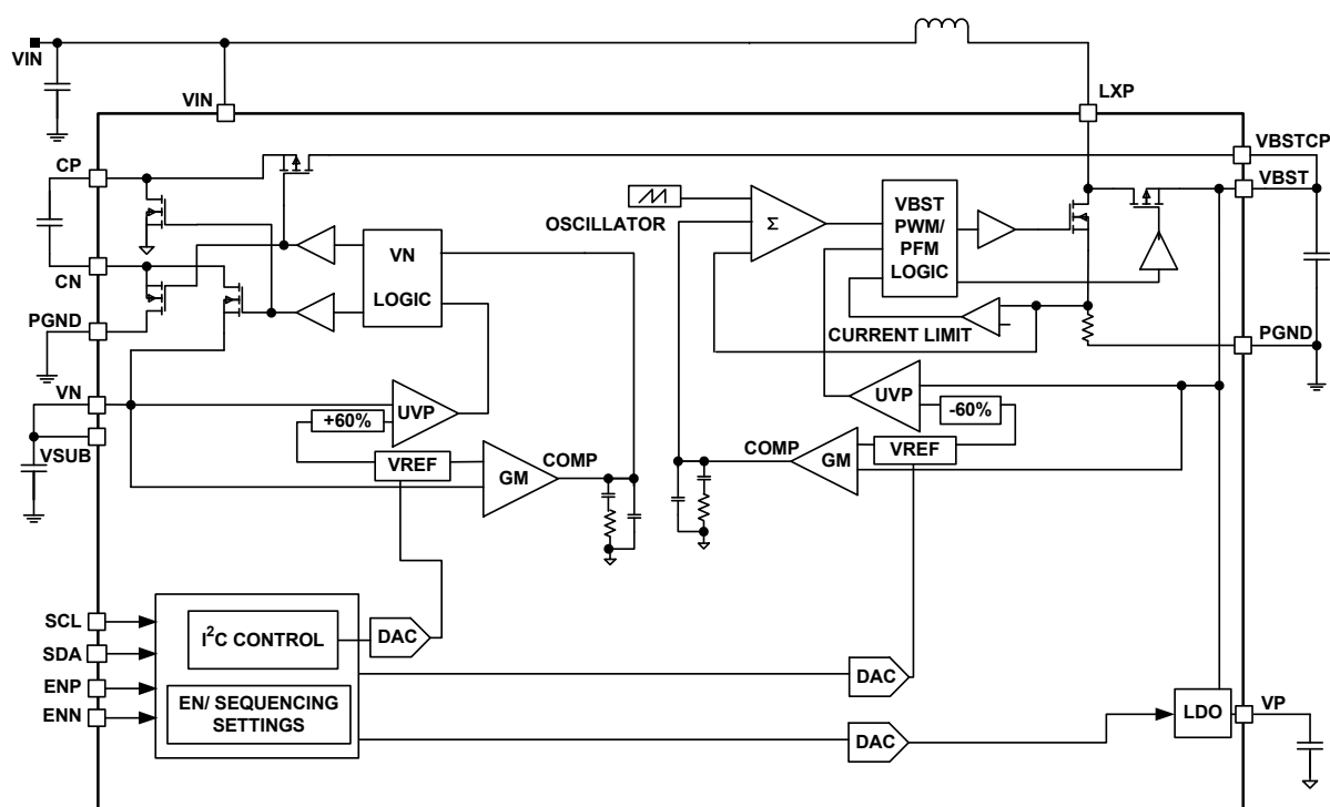
FIGURE 3. BLOCK DIAGRAM
