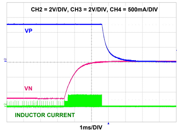
FIGURE 35. VP AND VN ( \pm 5\text{V} ) SHUTDOWN, VP/VN SEQUENCED (Reg 0x05 <b 4 > = 0)
