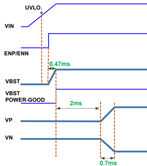
FIGURE 85. POWER-ON SEQUENCE – ACTIVATED BY ONE GPIO FOR ENN AND ENP, REGISTER 0x04 \langle b_4 \rangle = 1 AND 0x05 \langle b_7 \rangle = 1
