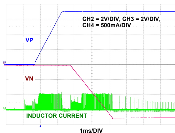
FIGURE 63. VP AND VN ( \pm 7\text{V} ) SOFT-START AT 5V INPUT VOLTAGE, VP/VN SEQUENCED (Reg 0x04 \langle b_4 \rangle = 0 )
