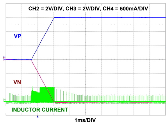
FIGURE 58. VP AND VN ( \pm 6\text{V} ) SOFT-START AT 3.7V INPUT VOLTAGE, VP/VN START TOGETHER (Reg 0x04 \langle b_4 \rangle = 1 )
