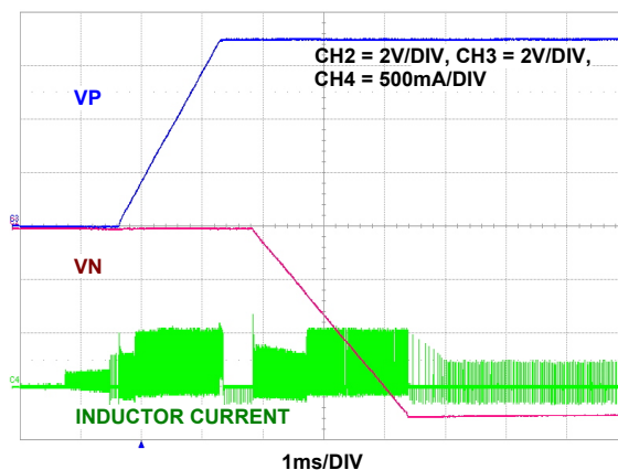
FIGURE 61. VP AND VN ( \pm 7\text{V} ) SOFT-START AT 2.5V INPUT VOLTAGE, VP/VN SEQUENCED (Reg 0x04 \langle b_4 \rangle = 0 )
