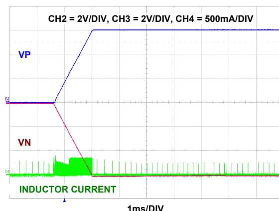
FIGURE 59. VP AND VN ( \pm 6\text{V} ) SOFT-START AT 5V INPUT VOLTAGE, VP/VN START TOGETHER (Reg 0x04 \langle b_4 \rangle = 1 )
