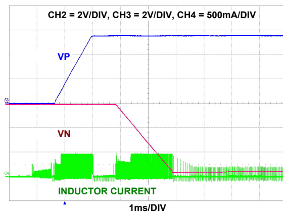
FIGURE 45. VP AND VN ( \pm 5.5\text{V} ) SOFT-START AT 2.5V INPUT VOLTAGE, VP/VN SEQUENCED (Reg 0x04 \langle b_4 \rangle = 0 )
