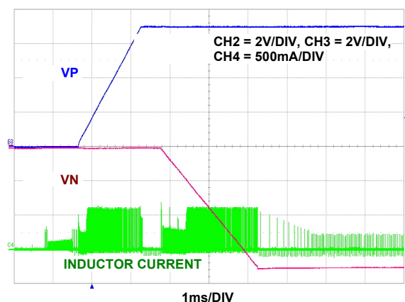
FIGURE 62. VP AND VN ( \pm 7\text{V} ) SOFT-START AT 3.7V INPUT VOLTAGE, VP/VN SEQUENCED (Reg 0x04 \langle b_4 \rangle = 0 )
