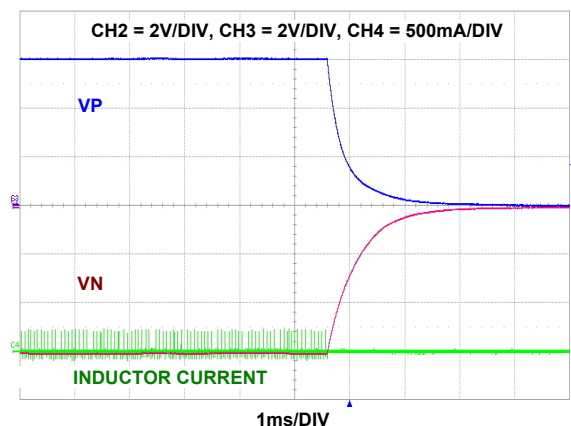
FIGURE 60. VP AND VN ( \pm 6\text{V} ) SHUTDOWN, VP/VN SHUTDOWN TOGETHER (Reg 0x05 \langle b_4 \rangle = 1 )
