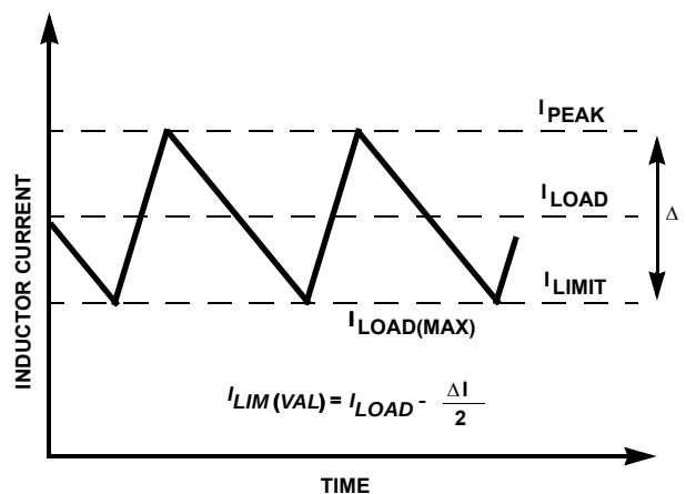
FIGURE 74. "VALLEY" CURRENT LIMIT THRESHOLD POINT
