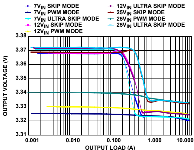
FIGURE 7. V_{OUT2} = 3.3V REGULATION vs LOAD (500kHz)
