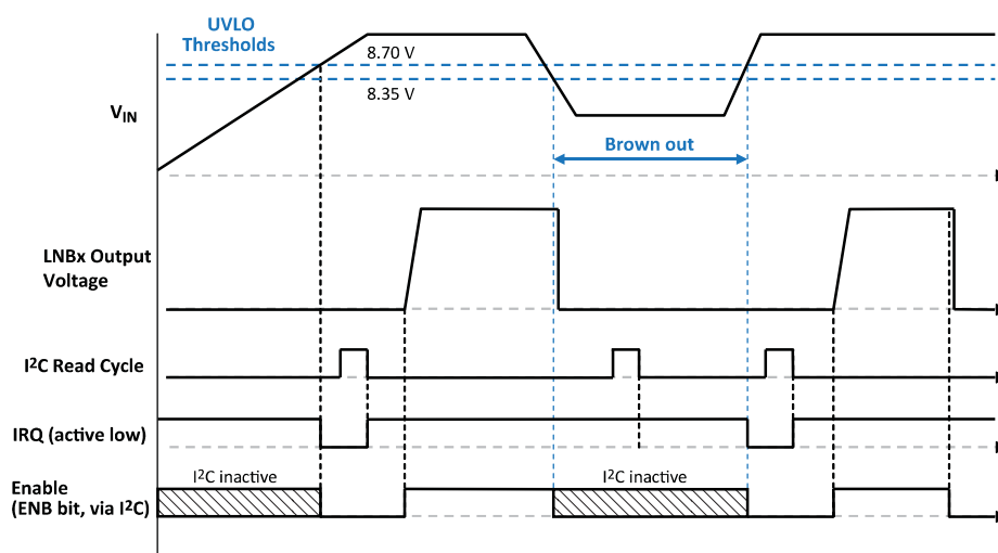
Figure 11. IRQ and Fault Clearing in Response to Undervoltage at VIN (UVLO). At power-up, while V_{IN} is below 8.70 V (typ), the A8299 is disabled and the I2C port is inactive. After V_{IN} rises above 8.70 V (typ), the I2C port becomes active and the IRQ pin is pulled low. An I2C Read is required to report and clear the UVLO fault and set the IRQ pin to a logic high before the A8299 can be enabled. If a brown-out occurs, such that V_{IN} drops below 8.35 V (typ), the A8299 will be disabled and the I2C port will become inactive (note that the IRQ pin will remain high during this time because the A8299 is disabled). After V_{IN} rises above 8.70 V (typ) the I2C port reactivates and the IRQ pin is pulled low to report that a brown-out had occurred. An I2C Read is required to report and clear the UVLO fault before the A8299 can be re-enabled.
