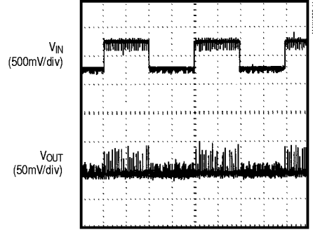
LINE-TRANSIENT RESPONSE
