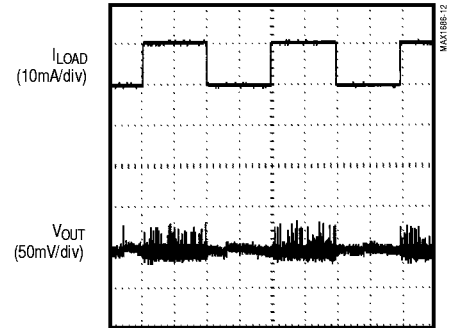
LOAD-TRANSIENT RESPONSE
