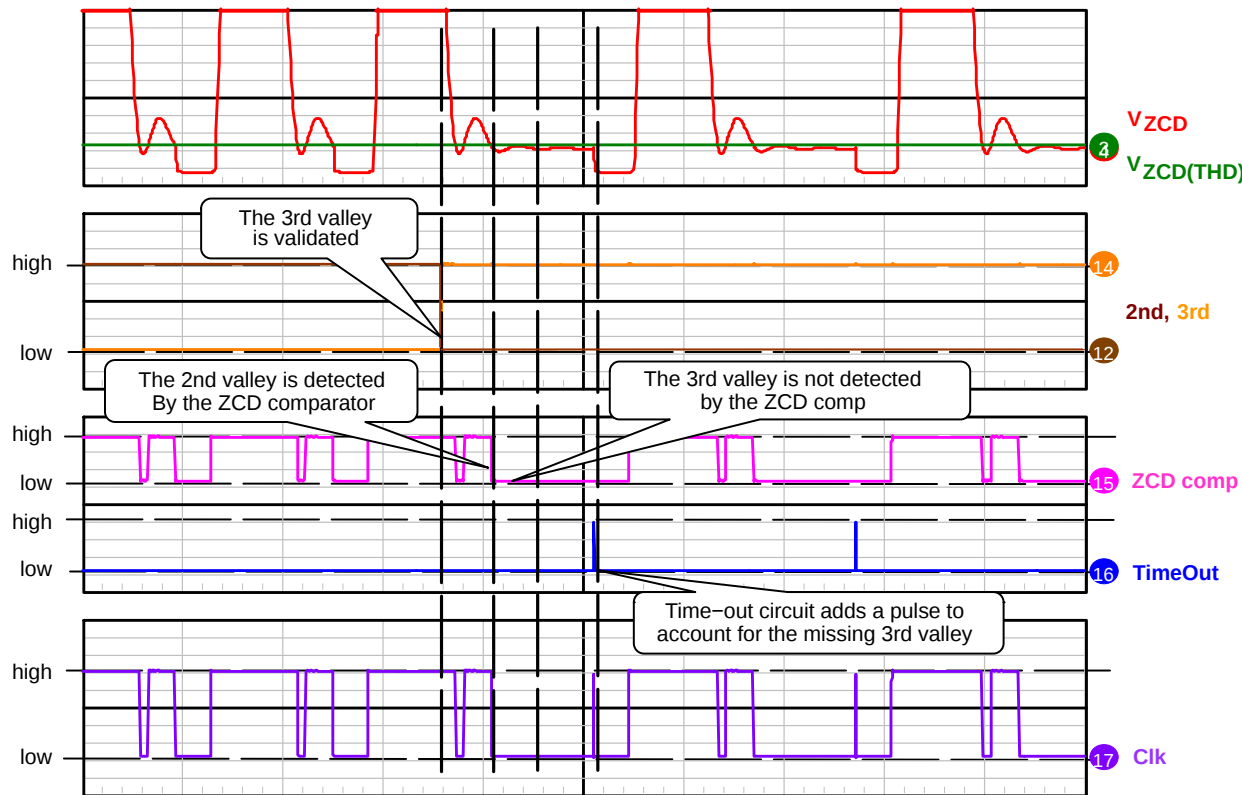
Figure 66. Time-out Chronograms
