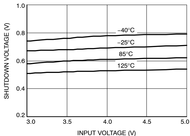
Figure 15. Shutdown Voltage
