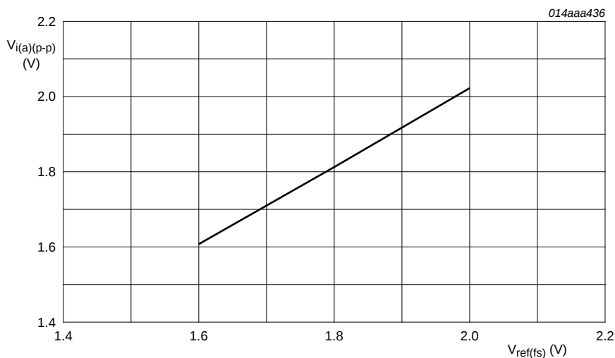
Fig 5. ADC full-scale; V_{i(a)(p-p)} as a function of V_{ref(fs)}
