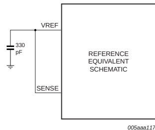
Fig 19. Internal reference, 1 V (p-p) full scale
